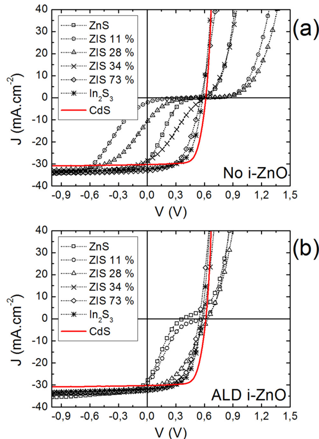
FIG. 8. J-V characteristics of solar cells with different buffer layers: (a) without any i -ZnO layer and (b) with an i -ZnO layer deposited by ALD.
