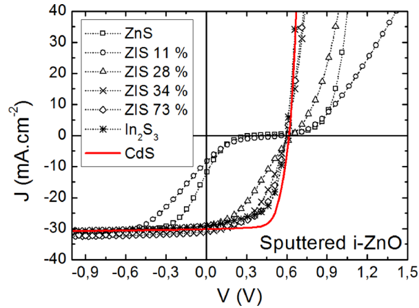
FIG. 5. Current density versus voltage (J-V) characteristics of solar cells as a function of the buffer layer composition with a sputtered i-ZnO layer. Illumination AM1.5 100 \text{ mW}\cdot\text{cm}^{-2} .
