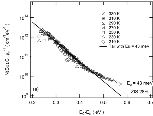
FIG. 4. Example of MPC density of states spectra for sample with ZIS of 28%.
