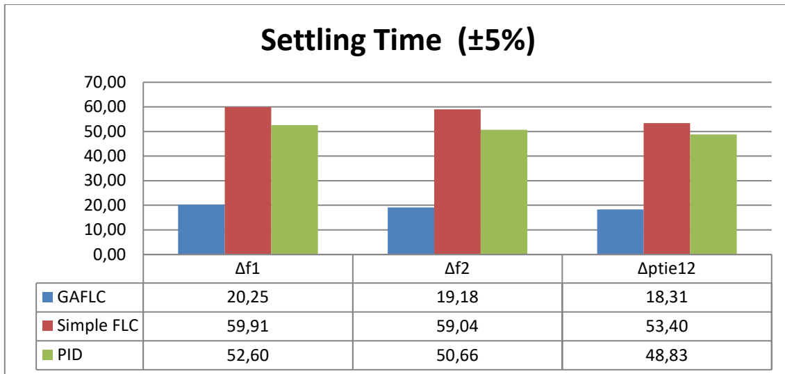
Figure 7 Settling Time comparison for different controllers
