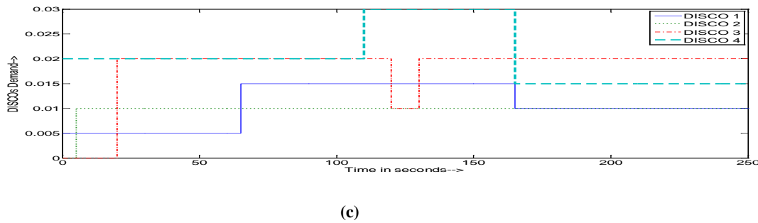
Figure 8 Comparison of GA optimized FLC, simple FLC and PID as per Test Case B (a) \Delta f_1 , (b) \Delta P_{tie12} and (c) demands of different DISCOs with respect to times
