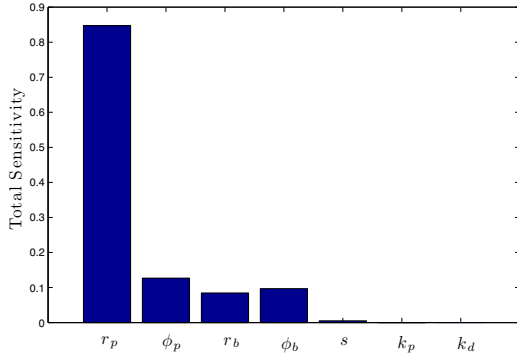
Fig. 6. Total effect-indices with fixed controller gains.
