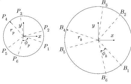
Fig. 2. Fixed base and movable platform.
