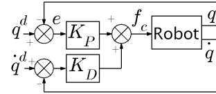
Fig. 3. Joint space PD controller of Stewart-Gough robot.
