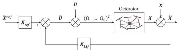
Fig. 5: Linear quadratic control for trajectory tracking
