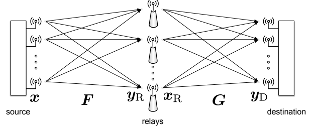
Fig. 1. The two-hop layered relay channel model.
