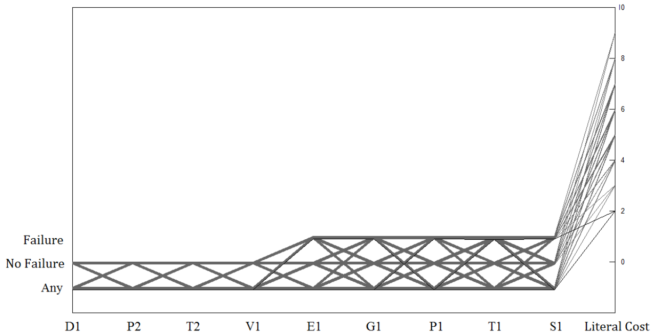
Fig. 10. Visualization of the results of the first iteration of the pruning step on the accident sequences of the CANDU AS
