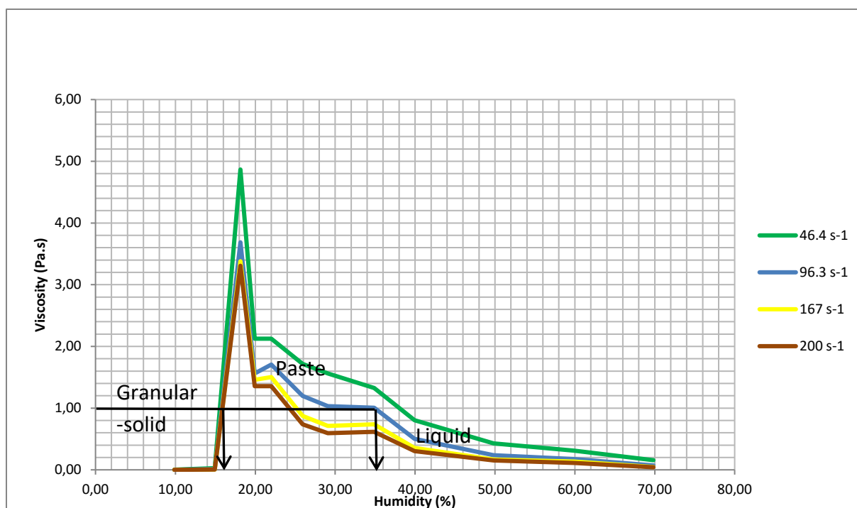
Figure 6: Evolution of the viscosity at four constant shear rates with different paste humidity levels.
