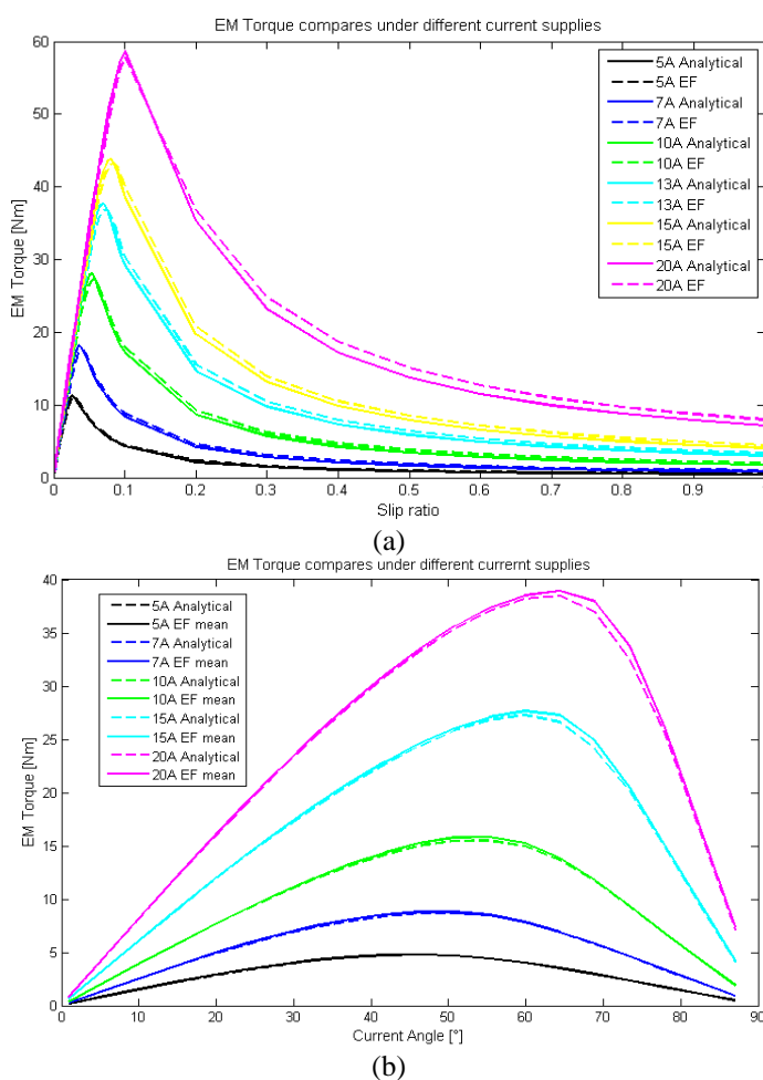
Fig. 2 Analytical model of (a) IM and (b) SRM validated by FEM
