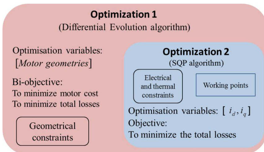
Fig.3 Global optimization scheme
