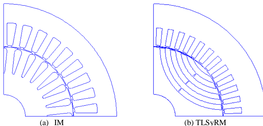
Fig. 1 Geometrical Structure of studied machines
