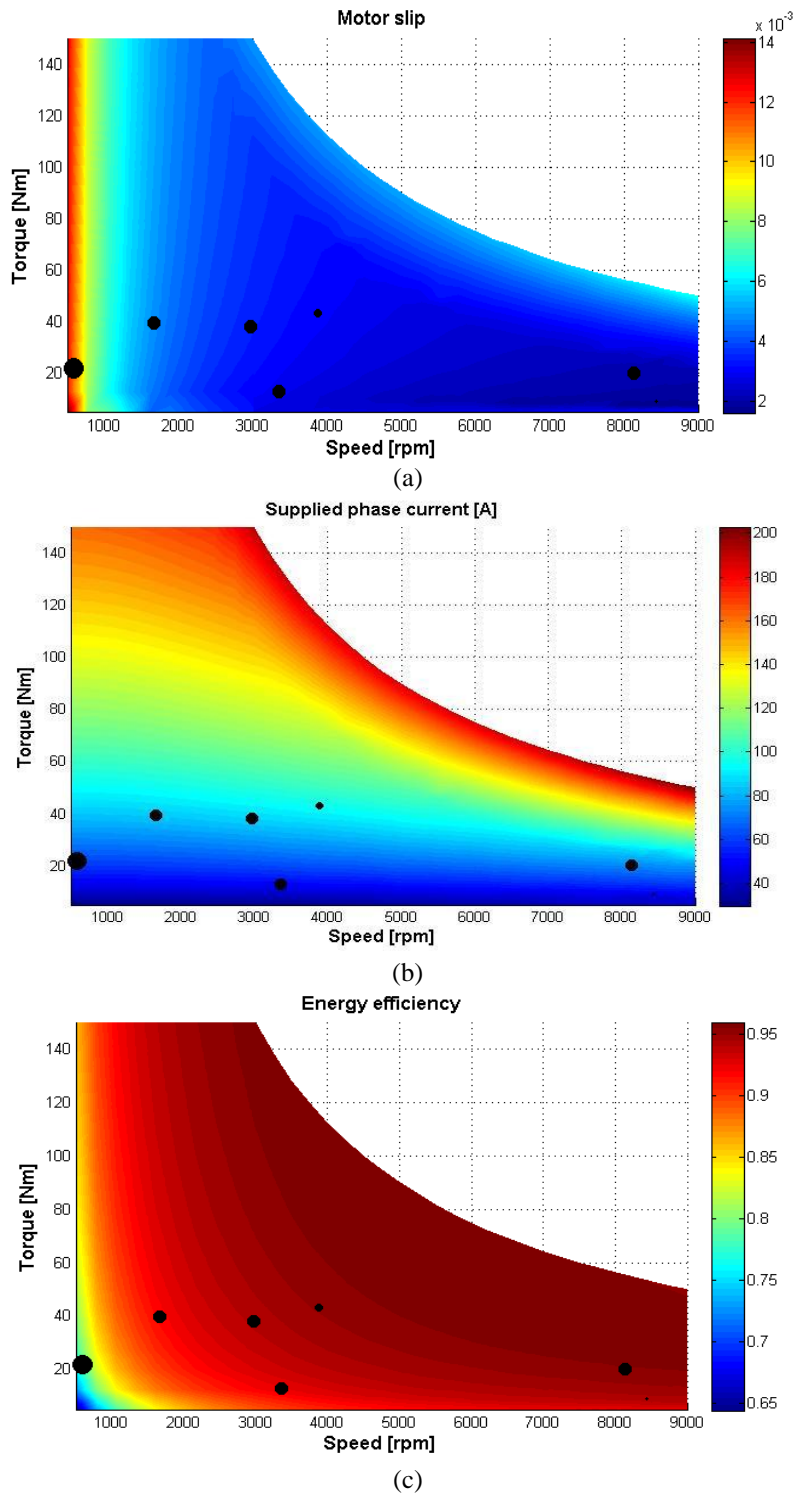
Fig.4 Optimal command parameters (slip ratio (a) and phase current amplitude (b)) (c) Optimal energy efficiency with electrical constraints of an optimized four-pole IM
