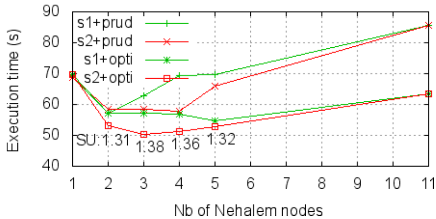
Figure 9: Exec. time of cl3 benchmark on our Nehalem cluster
