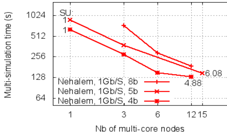
Figure 13: c13 benchmark time with 4, 5 and 8 buildings on 1Gb/s cluster
