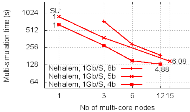
Figure 13: c13 benchmark time with 4, 5 and 8 buildings on 1Gb/s cluster
