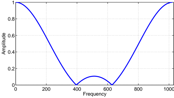
Figure 1: Amplitude Response of Proakis C Channel.
