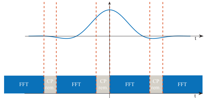
Fig. 4: Demodulation operations at the CP-OFDM receiver with an interfering OFDM/OQAM signal. The well-shaped PHYDYAS filter is cut in small non-contiguous parts on which FFT operations are performed.
