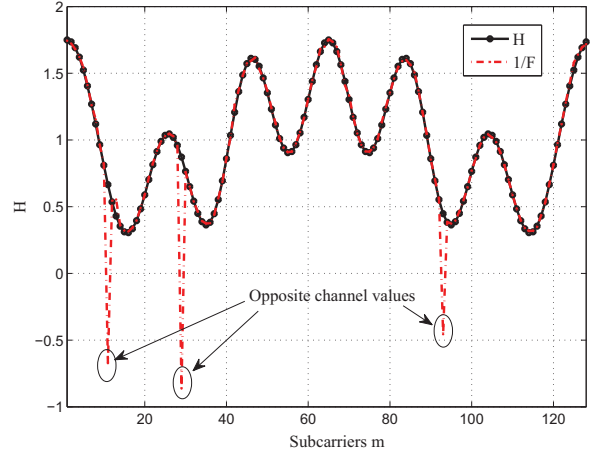
Fig. 1. Real part of H and 1/F showing opposite equalizer coefficient values.
