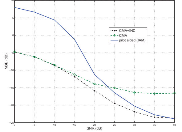
Fig. 5. MSE performance versus SNR. Comparison between CMA, CMA using IN cancellation (ICN) with sub-optimal initialization value, and pilot-aided method (IAM).
