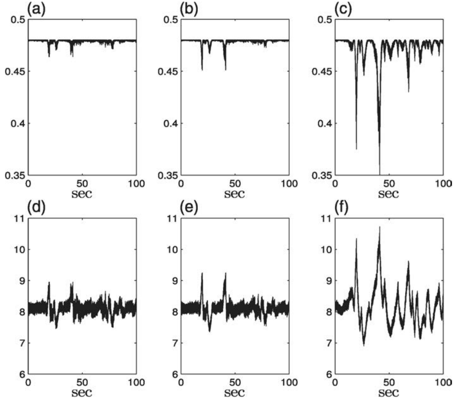
Figure 6. (a), (b), and (c) power coefficient C_p in gradient dynamics-block-backstepping controller, PI controller, and standard passivity-based controller, respectively. (d), (e), and (f) TSR \lambda in the same controllers.
