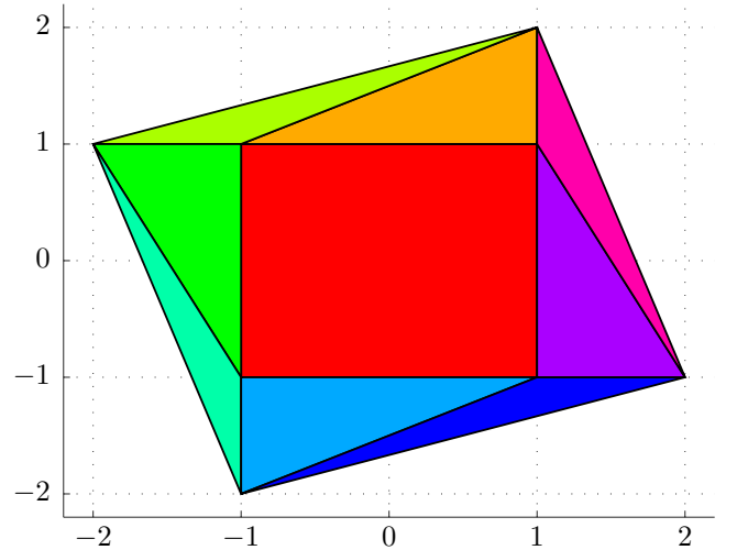
Fig. 1: A cell complex of a polytope in \mathbb{R}^2 .
