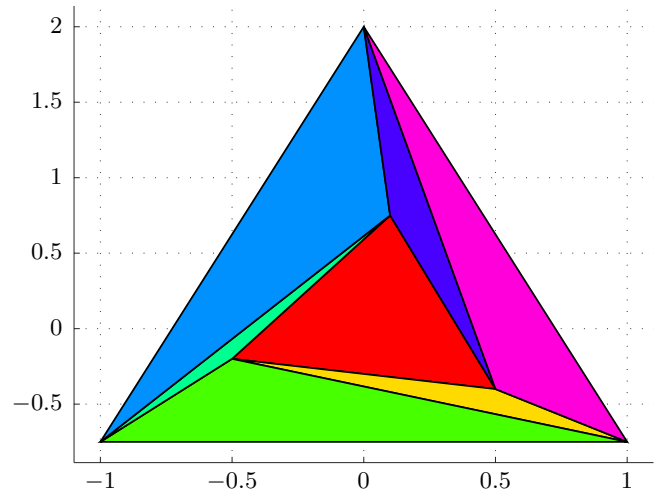
Fig. 5: A convexly non-liftable cell complex in \mathbb{R}^2 .
