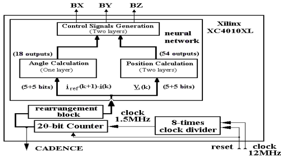
Fig. 22: ANN structure and testbench for operation speed testing
