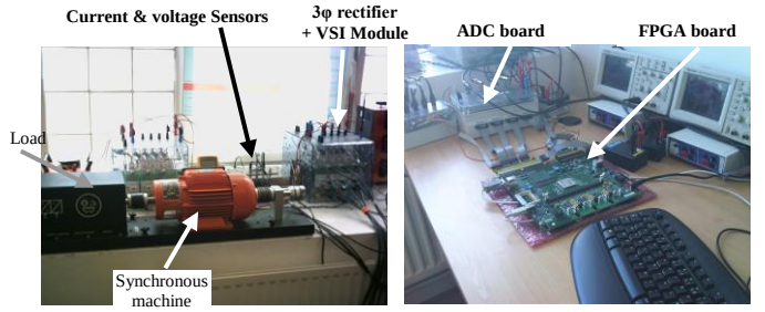
Fig. 18. Prototyping platform
