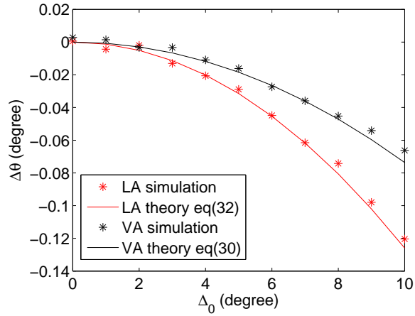
Figure 5: DOA estimation error vs. the source angular extension \Delta_0 (LA with M = 20 and d = \lambda/4 , VA with M = 20 and d = \lambda/4 and \beta = 100^\circ , one source with uniform angular dispersion with \theta = 45^\circ , \Delta_0 = 2\sqrt{3}\sigma )
