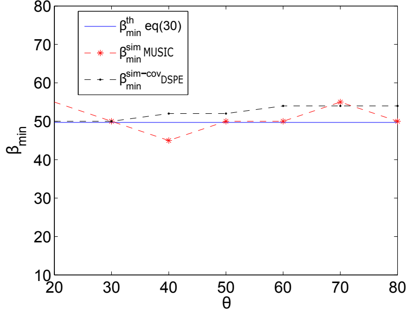
Figure 4: Value of \beta corresponds to the minimum value of: 1) the theoretical expression of |\Delta\theta| in eq(30), 2) the |\Delta\theta| obtained by the simulation with MUSIC 3) the covariance of \theta and \sigma of DSPE (simulation), (VA with M = 10 and d = \lambda/2 , one source with uniform angular dispersion, \Delta_0 = 10^\circ )
