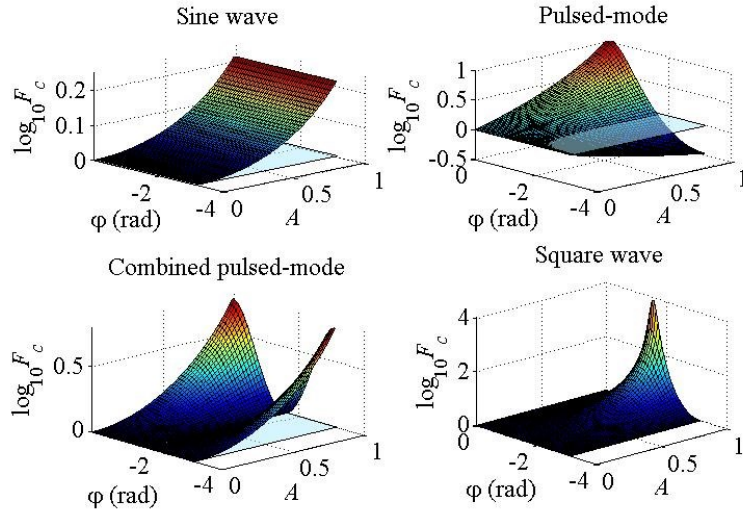
Fig. 4. Amplification factor for the four actuation waveforms. The light-blue surface corresponds to \log_{10}(F_c(A, \phi))=0 .
