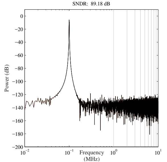
Figure 10. ADC output spectrum
