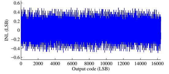
Figure 9. INL of proposed ADC
