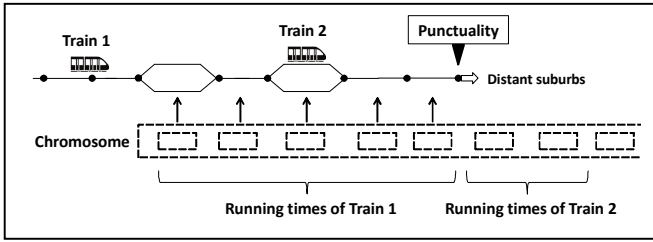
Fig. 1. Chromosome coding.
