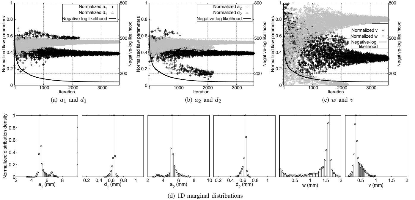
Fig. 11. Normalized N -MultiNest samples, negative-log likelihoods vs. iterations and 1D marginal distribution densities for the double-crack model at v = 0.3 mm, SNR = 20 dB. Normalizations are performed with respect to the parameter ranges given in Tab. III.
