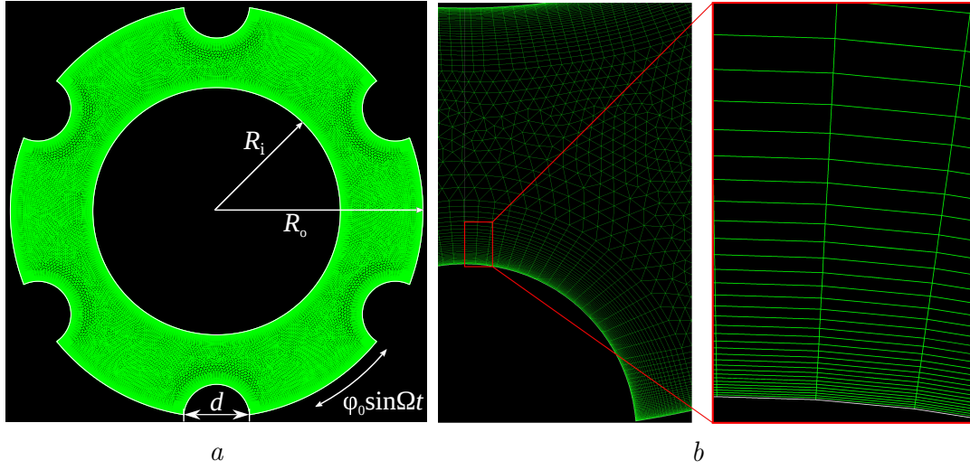
Figure 2. Annulus with deflectors with the grid meshed for the frequency 4 Hz (a); R_i – inner radius, R_o – outer radius, d – activator diameter. The figure (b) is zoomed: adaptive mesh is seen in the boundary zone on the walls
