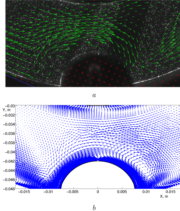
Figure 11. Velocity field near an activator at f = 4.0 \text{ Hz} and \varphi_0 = 0.06 \text{ rad} ( \text{Re}_p = 226 , \omega = 1608 ); symmetry break is observed ( a – experiment, Q_a = 21.0 \pm 0.8 \text{ mm}^2/\text{s} , the vortex B is “even”; b – simulation, Q_a = 15.5 \text{ mm}^2/\text{s} , the vortex B is “odd”)
