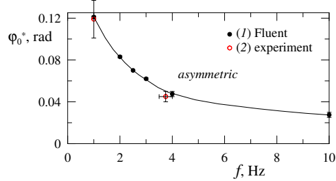
Figure 13. Stability threshold from numerical simulation (1) and from experiment (2)
