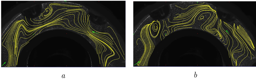
Figure 14. Streamlines traced based on PIV data for f = 4.0 Hz, \varphi_0 = 0.06 rad (a) and 0.09 rad (b). The cog-wheel vortex is regular in figure (a), at the higher amplitude it undergoes an instability (b)
