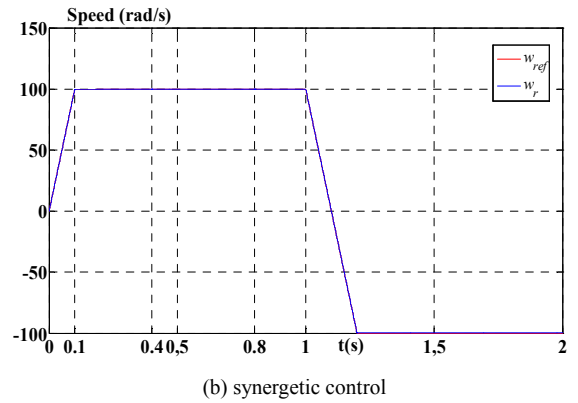
Figure 3. Speed responses of a PMSM controlled by sliding mode and synergetic.
