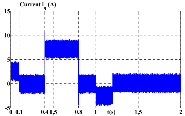
(a) sliding mode control.
