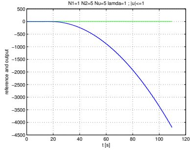
Fig. 5: Reference tracking designed by GPC with N_2 = 5 .
