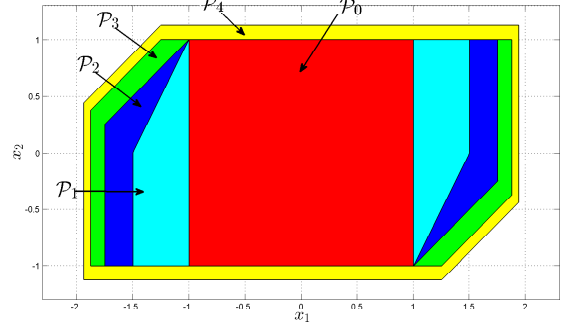
Figure 5: Sequence of the forward mappings \text{Conv}(\mathcal{P}, A_0\mathcal{P} \oplus A_d\mathcal{P}) , for the Example 1.
