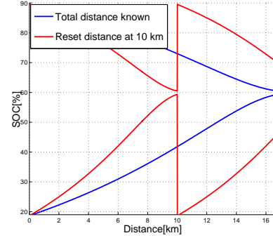
Fig. 3. SOC limits for 2 cases: total distance known and reset distance fixed at 10 km, respectively
