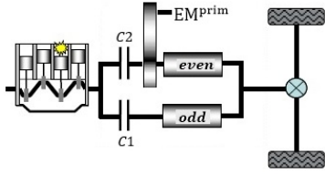
Fig. 1. DCT hybrid configuration
