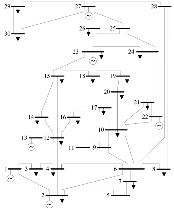
Fig. 3. Single-line diagram of the IEEE 30-bus test system.
