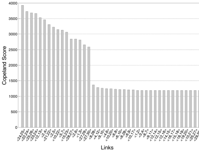
Fig. 8. Copeland score ranking of the resilience reduction worth R_{RRW_{ij}}(\Delta t_0 = 3) for all IEEE 30-bus network links.
