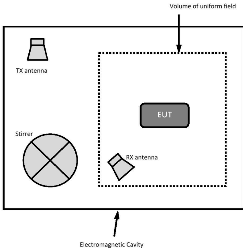
Fig. 1. Typical RC facility.
