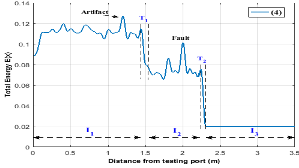
Fig. 2. The energy diagram produced after applying DORT on the DJ NUT of Fig. 1 with two testing ports at {1} and {3} observed along the third path.
