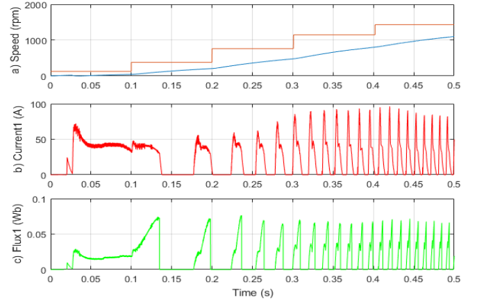
Fig. 9. Speed, phase current and flux linkage waveforms
