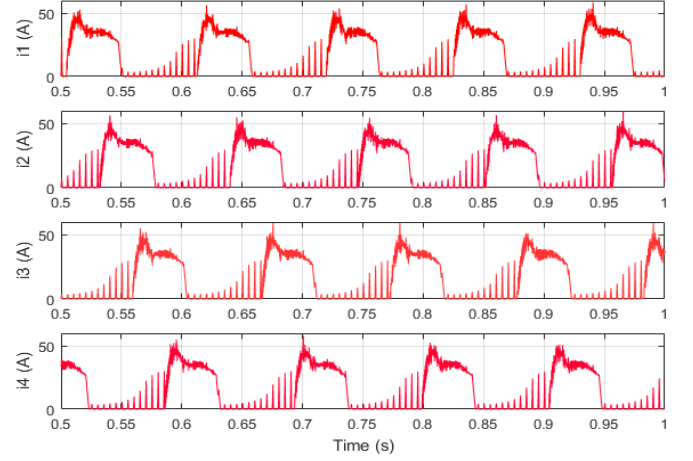
Fig. 5. Four-phase current waveforms
