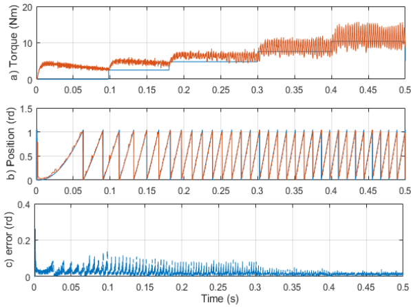
Fig. 11. Electromagnetic and load torque, actual and estimated position, position error
