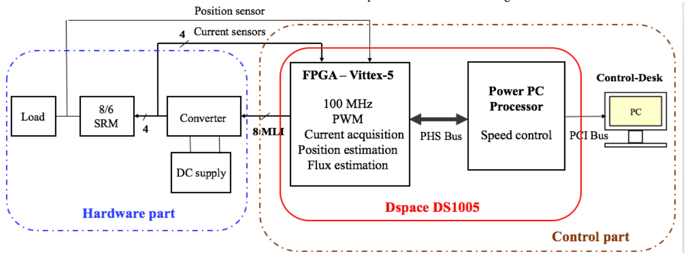
Fig. 12. Block diagram of the SRM experimental setup
