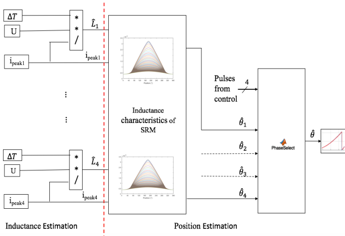
Fig. 4. Block diagram for the four-phase SRM position estimation
