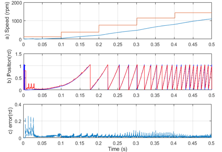
Fig. 10. Speed, actual and estimated position, position error
