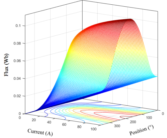
Fig. 1. Flux-linkage characteristics of SRM
