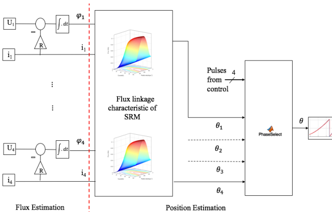
Fig. 8. Position estimation based on flux linkage computation
