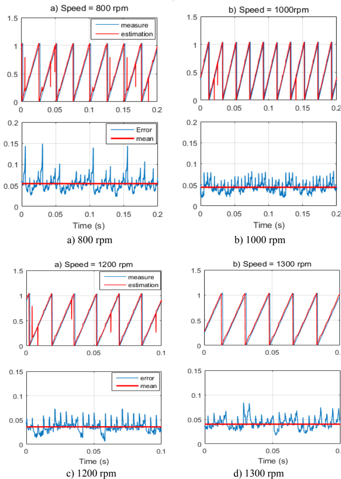
Fig. 14. Position estimation experimental results with flux-based method
