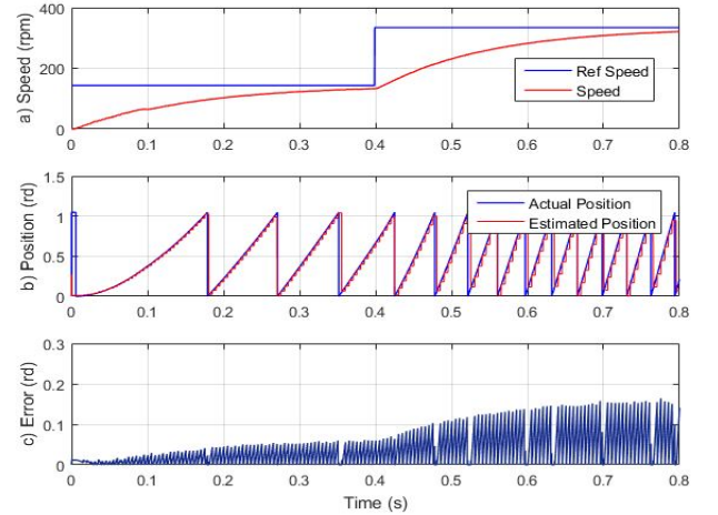
Fig. 6. Influence of the speed
