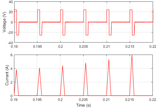
Fig. 3. Principle of pulse injection
