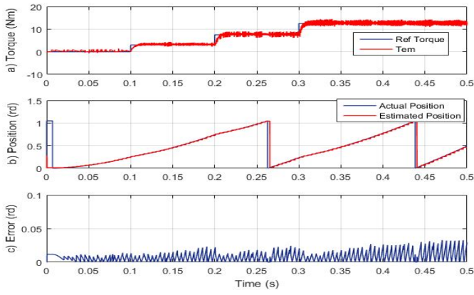
Fig. 7. Influence of the load torque
