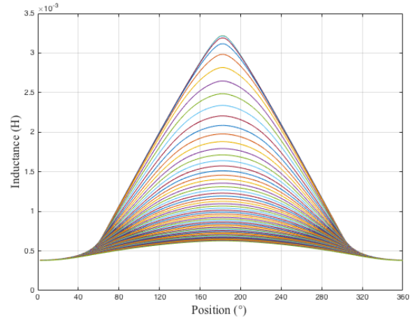
Fig. 2. Inductance characteristics of SRM
