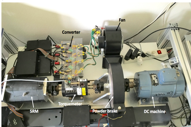
Fig. 13. Experimental SRM drive
