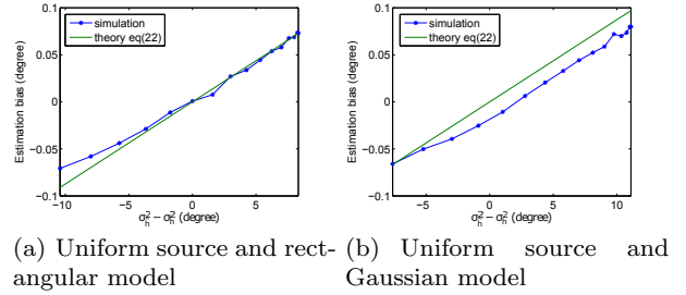
Fig. 2 DOA estimation error vs. difference of the angular spread between signal and model. (1 source)
