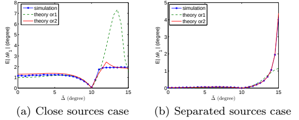
Fig. 5 |E[\Delta\theta_1]| vs. model angular dispersion \tilde{\Delta} (2 sources)
