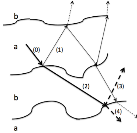
Figure 1: First successive sets of internal and external scattering events.
