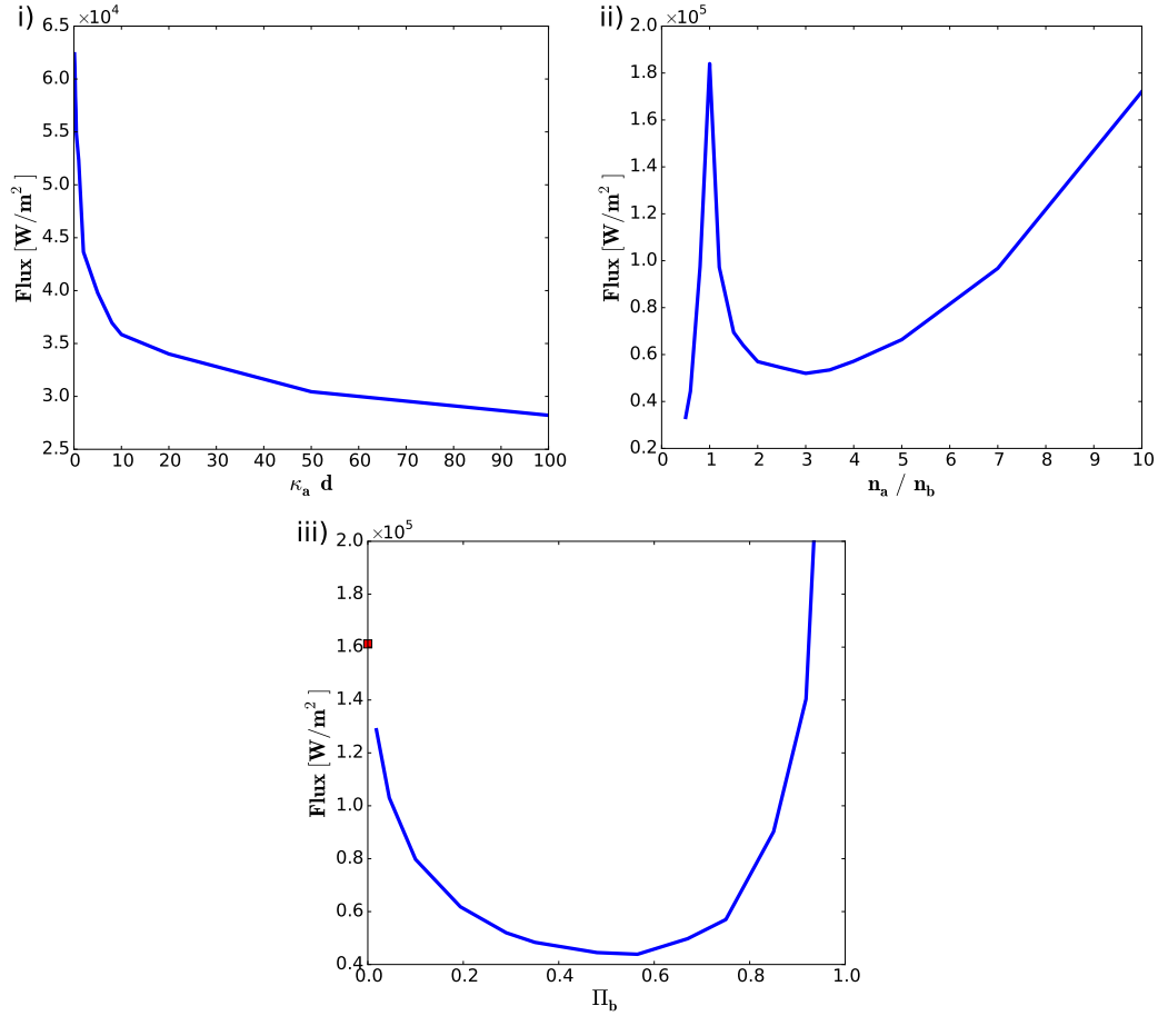
Figure 11: Radiative flux through the fibrous medium: i) vs absorption optical thickness; ii) vs optical index ratio; iii) vs porosity; The medium is bounded by two black walls at T(0) = 2000K and T(D) = 300K ; Other parameter values are: \kappa_a d = 0.3 , n_a/n_b = 2 , \Pi_b = 0.75 .
