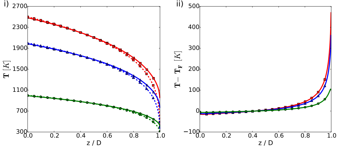
Figure 9: i) Temperature field when the fibrous medium is bounded by two black walls; \square : T(0) = 2500K , \triangle : T(0) = 2000K , \circ : T(0) = 1000K ; In all cases: T(D) = 300K .; (- - -) coupled GRTEs model, ( \cdots ) Fourier's model associated with coupled RTEs; ii) Residuals.
