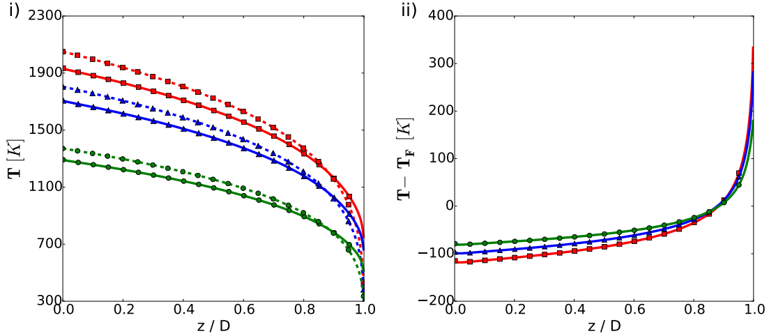
Figure 10: i) Temperature field when a fibrous medium is submitted to an imposed flux at z = 0 and bounded by a black wall at z = D ; \square : \varphi(0) = 50 kWm^{-2} , \triangle : \varphi(0) = 30 kWm^{-2} , \circ : \varphi(0) = 10 kWm^{-2} ; T(D) = 300K ; (- - -): coupled GRTEs model, ( \cdots ): Fourier's model associated with coupled RTEs; ii) Residuals.
