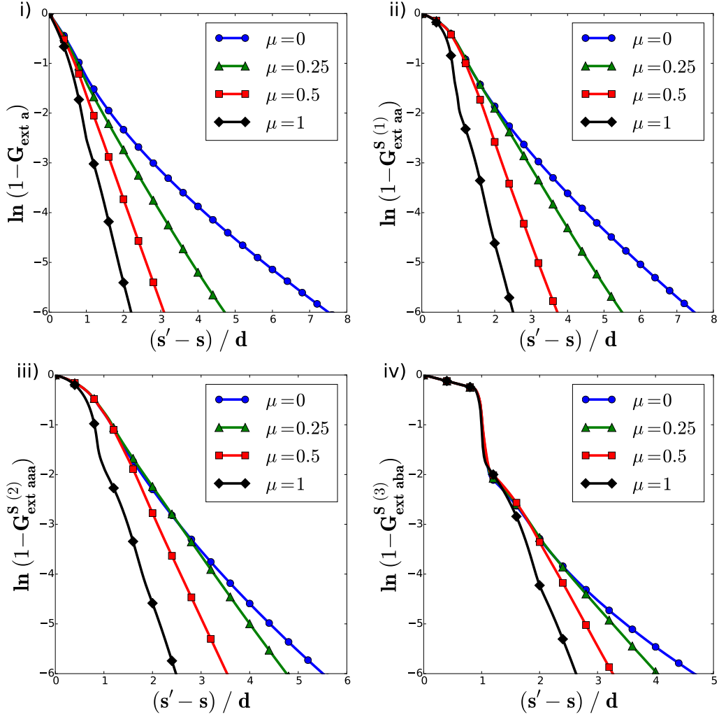
Figure 5: Extinction cumulative distribution functions of phase a (fibres) for different values of \mu = \cos \theta . i) G_{ext a} associated with isotropic volume emission points; ii) G_{ext aa}^S(1) ; iii) G_{ext aaa}^S(2) ; iv) G_{ext aba}^S(3) (by using notations of Sec.2.1.1 and Fig.3.)
