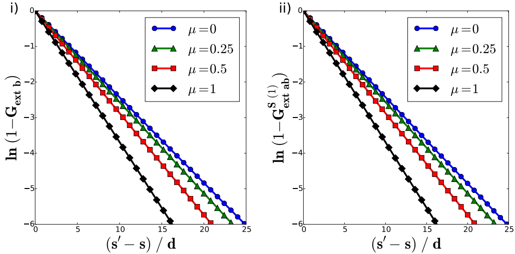
Figure 4: Extinction cumulative distribution functions of the transparent phase b for different values of \mu = \cos \theta : i) G_{ext b} associated with isotropic volume source points; ii) G_{ext ab}^{S(1)} associated with interfacial scattered rays (path 2 of Fig.3).
