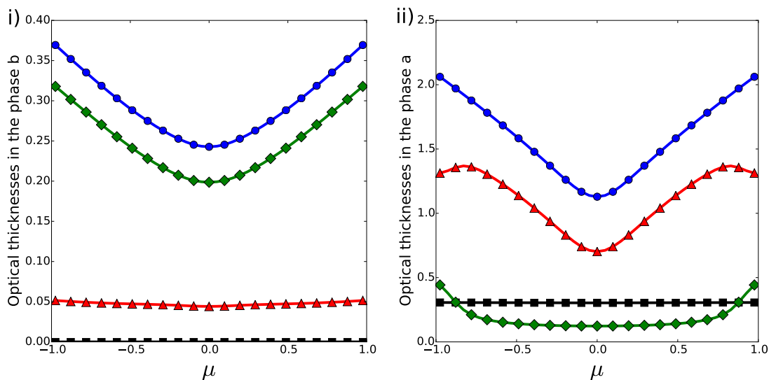
Figure 6: Optical thicknesses based on \circ : Generalised extinction coefficients ( B_c d ); \triangle : Generalised internal scattering coefficients ( \Sigma_{cc} d ); \diamond : Generalised external scattering coefficients ( \Sigma_{cd} d ) and \square : Absorption coefficients ( \kappa_a d = 0.3 and \kappa_b d = 0 ); i) For the transparent phase b ( c=b , d=a ); ii) For the absorbing phase a (fibres) ( c=a , d=b ).
