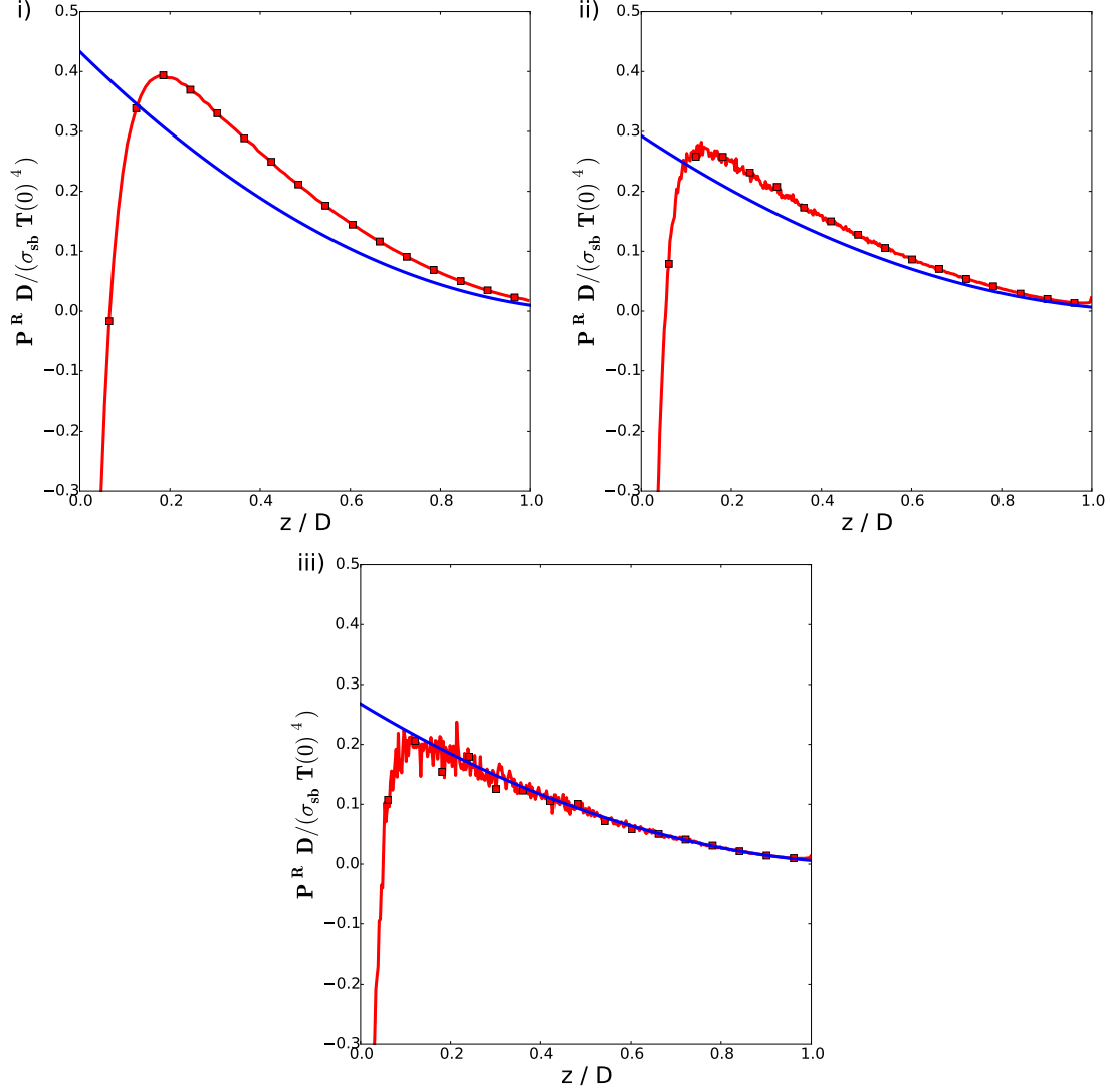
Figure 8: Dimensionless radiative power field for an imposed linear temperature field in the fibre phase; Two boundary black walls at T_a(0) = 2000K and T_a(D) = 300K : i) \kappa_a d = 0.3 ; ii) \kappa_a d = 10 ; iii) \kappa_a d = 100 ; \square : coupled GRTEs model, - : Fourier's model associated with coupled RTEs.
