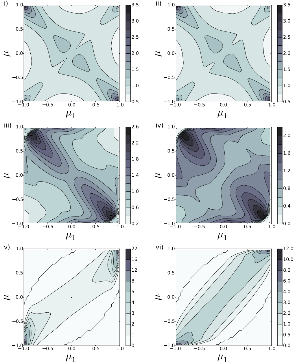
Figure 7: Phase functions. i) p_b(\mu_1, \mu) , internal scattering within b (Beerian model, random volume source points); ii) p_{abb}(\mu_1, \mu) internal scattering within b following transmission from a (interfacial source points); iii) p_{aa}(\mu_1, \mu) first internal scattering within a; iv) p_{aaa}(\mu_1, \mu) (second internal scattering within a; v) p_{ba}(\mu_1, \mu) , external scattering from b to a (Beerian model, random volume source points); vi) p_{ab}(\mu_1, \mu) (first external scattering from a to b).
