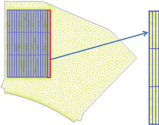
Figure 17. Geometry configuration 18 vertical turns-Each conductor is a 9 strands Litz wire (Version 1)
