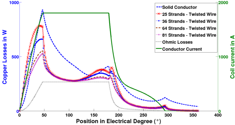
Figure 10. Copper losses in case of twisted wire conductor for multiple numbers of strands
