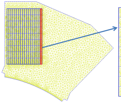
Figure 19. Geometry configuration 18 vertical turns-Each conductor is a 9 strands Litz wire (Version 2)
