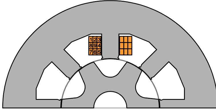
Figure 2. Position of the 9 parallel strands and the machine cross section
