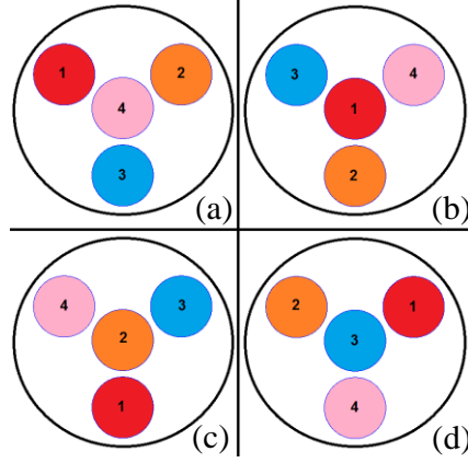
Figure 6. Strands positions throughout a weaving pitch with a length of \Delta l along the z -axis. a) 0 < z \leq \frac{\Delta l}{4} ,
