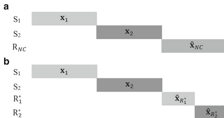
Fig. 2 Time allocation. a Network coding-based cooperation—one relay is selected which forwards the whole network-coded codeword to help the two sources simultaneously. b Partial relaying-based cooperation—two relays are selected, each forwarding half of estimated codeword to help one source independently
