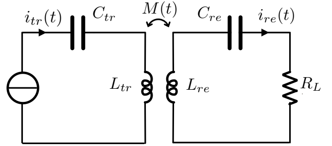
Fig. 5: Circuit representation of the analyzed configurations.
