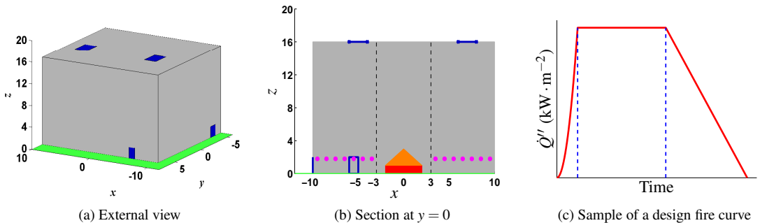
Fig. 4. (a) External view of the considered building. (b) Section of the building. The triangle in the middle is the fire, the bullet points are the sensors. (c) Time evolution of the Heat Release Rate.
