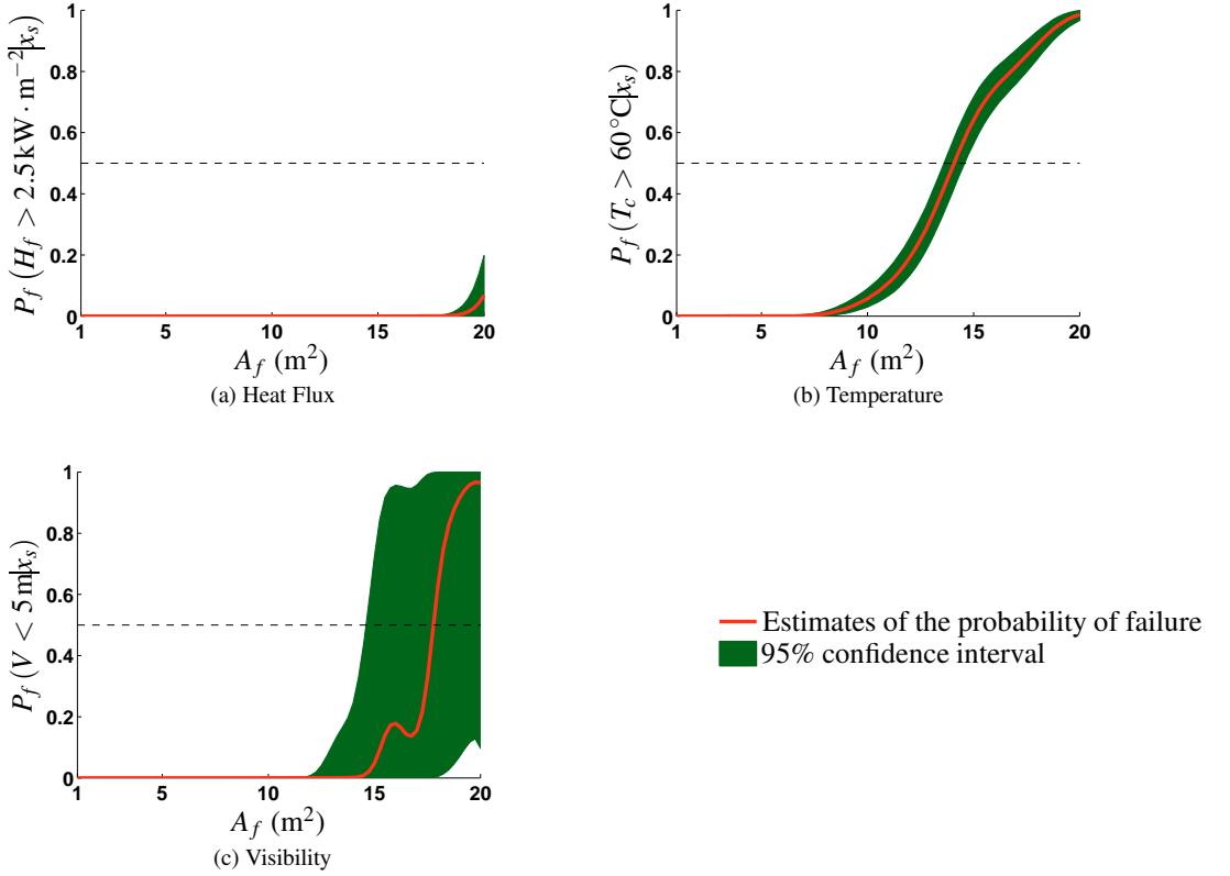
Fig. 6. Estimates of probabilities of failure as function of the scenario variable A_f \in [1; 20] \text{ m}^2 , the fire area. Each figure corresponds to one output: (a) Heat Flux H_f , (b) Temperature T_c and (c) Visibility V .
