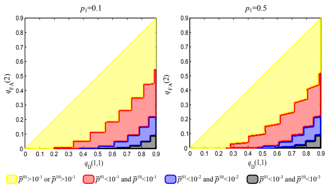
Fig. 12. Achievable \bar{p}^{10} or \bar{p}^{01} for different values of the pair (q_D(1,1), q_{FA}(2)) when p_1 = 0.1 (left) and for p_1 = 0.5 (right) and p_2 = 0 .
