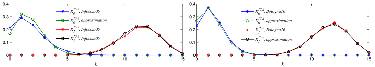
Fig. 5. Values of X_\theta^{15,k} the end of the simulation, as well as the theoretical values at equilibrium obtained from (19), obtained using the Infocom05 database (left) and the Bologna16 database (right).
