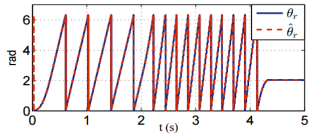
c. Actual and estimated rotor position
