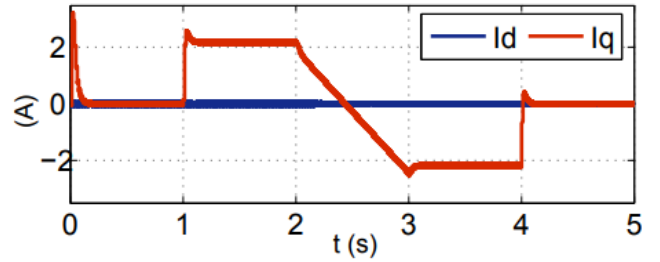
Fig.7. Park Transformed currents i_d, i_q In the following, the robustness of the simplified HFI is evaluated against parameter variation with \pm 50\% variation introduced in the stator resistance R_s . The simulation results of the speed, position and the estimation errors displayed in figure 8 show that the estimation efficacy is not altered.
