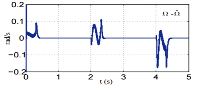
b. Rotor speed estimation error
