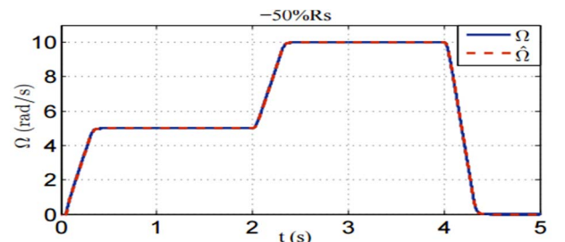
c. Actual and estimated speeds with -50%Rs
