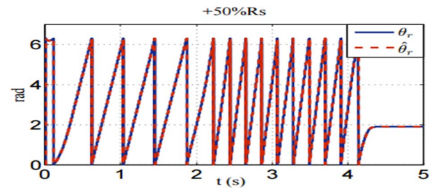
b. Actual and estimated position with +50%Rs
