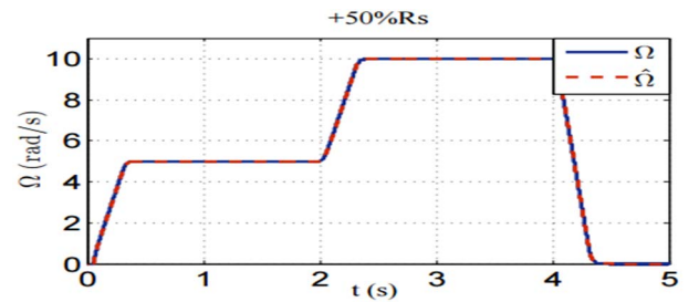
a. Actual and estimated speeds with +50%Rs
