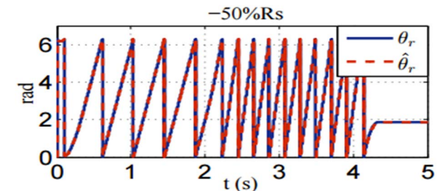
d. Actual and estimated position with -50%Rs
