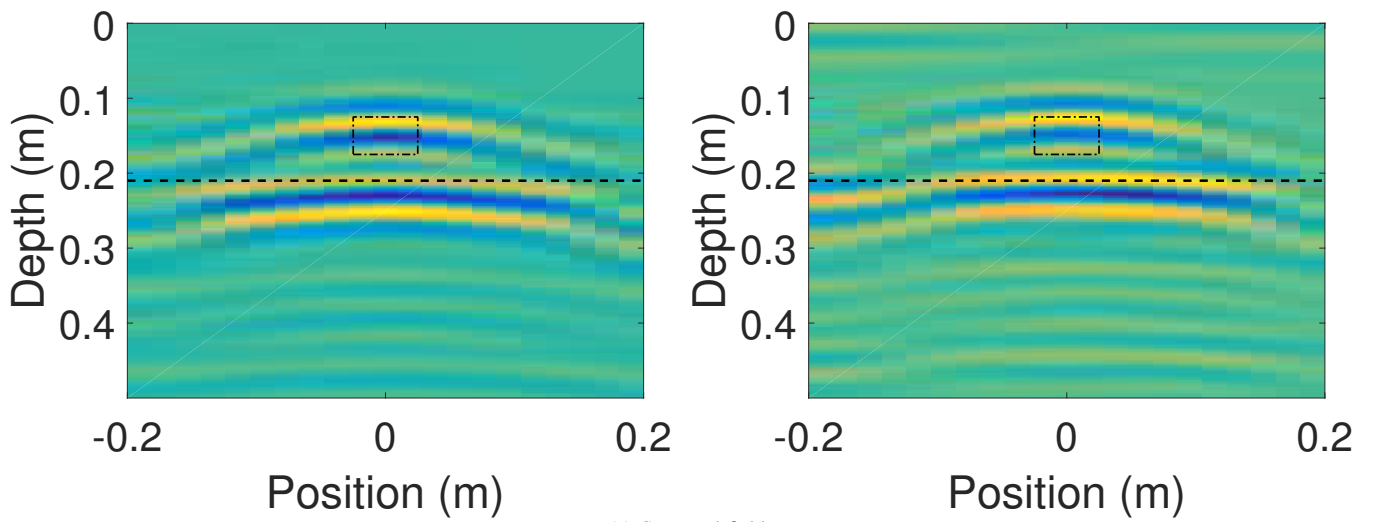
(c) Scattered field
