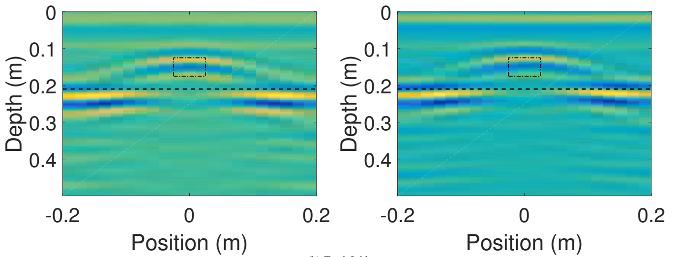
(b) Total field
