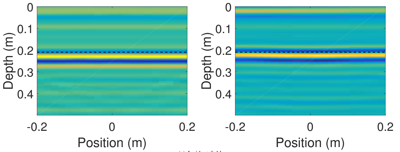
(a) Incident field
