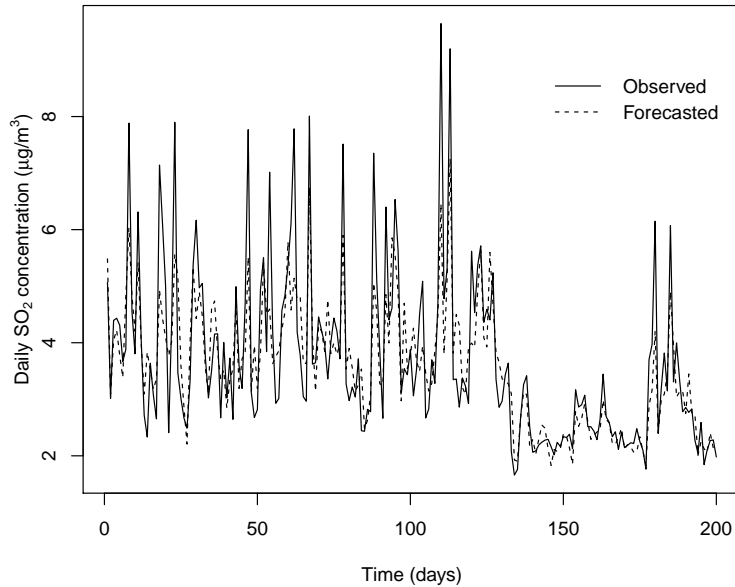
Figure 10: Forecasted values by the robust SARFIMA model and \text{SO}_2 concentrations ( \mu\text{g}/\text{m}^3 ) from June 15th 2009 to December 31st 2009, one-step-ahead.
