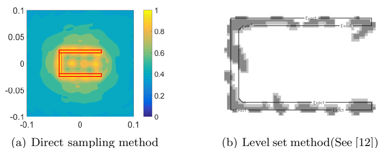
Figure 4. Comparison between DSM and Level set method with experimental data at 8 GHz
