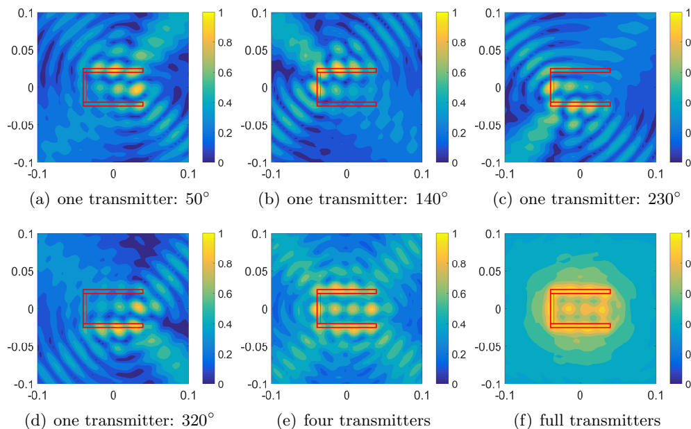
Figure 2. Imaging results of experimental data: Single-frequency DSM at 8 GHz
