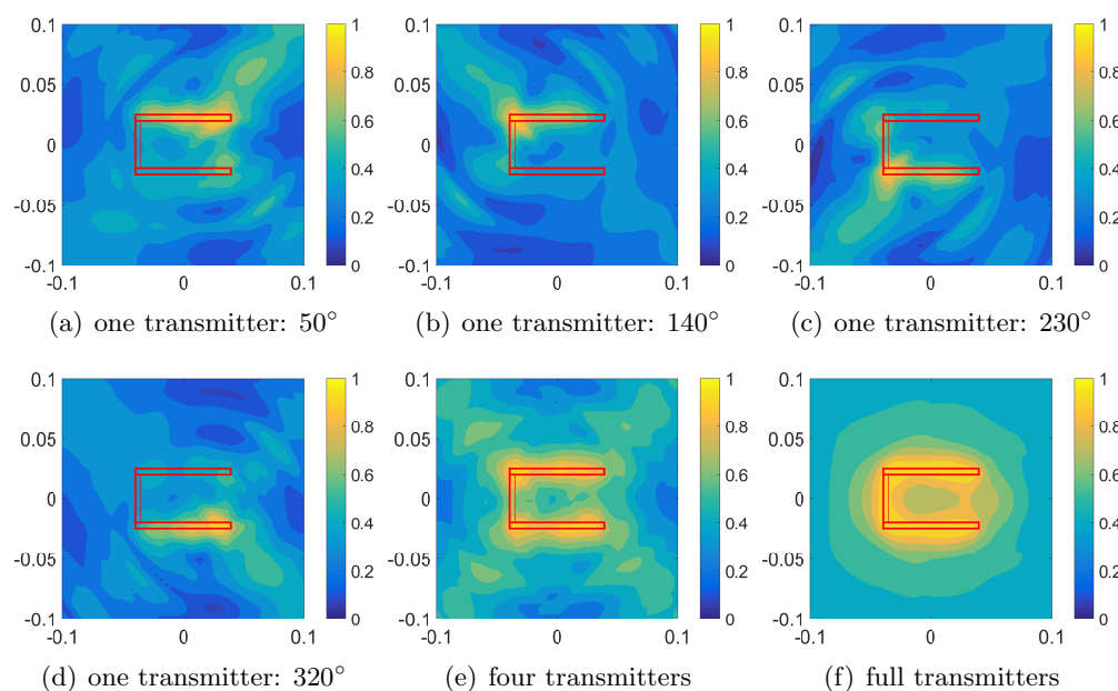
Figure 3. Imaging results of experimental data: Multi-frequency DSM
