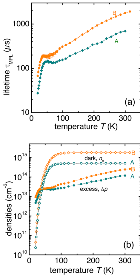
Figure 3 In (a), MPL lifetimes of samples A and B versus T are shown. For sample B the mean values and error bars are determined from four consecutive measurements from two down/up-cycles in T . For most of the temperatures the error bars are smaller than the symbol size. In (b), the densities \Delta p (= \Delta n) , determined from the MPL lifetimes and n_0 of samples A and B versus T are shown.
