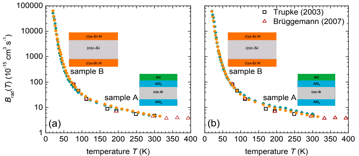
Fig. 4. Determined B_{rad} values for the two samples A and B together with data from [1] and [2]. The absolute B_{rad} values are based on calibration with data from [1] at 300 K in (a) and at 90 K in (b).
