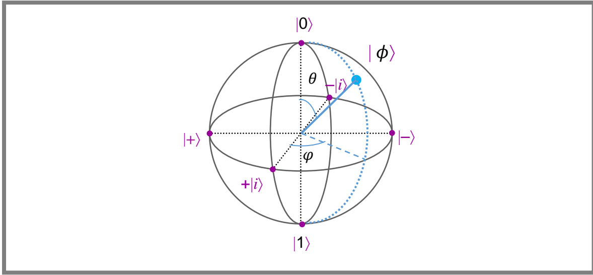
Figure 1. Bloch sphere with the qubit state |\phi\rangle characterized by the angles \theta and \varphi .
