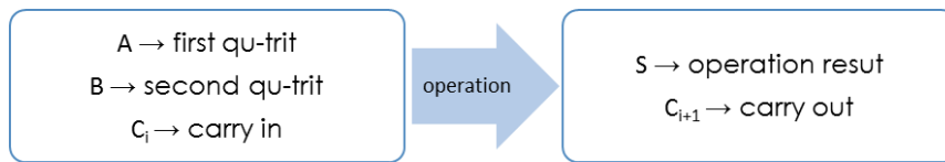
Figure 2. General arithmetic operation diagram in a qu-trit system.
