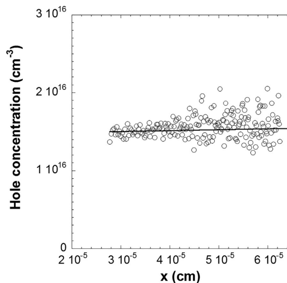
Figure 5. The concentration profile from C–V measurements for the n-GaP/p-Si heterostructures grown on p-Si boron doped substrates using hydrogen plasma (20 W).
